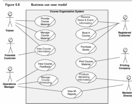
Figure 6.8 Business use case model
